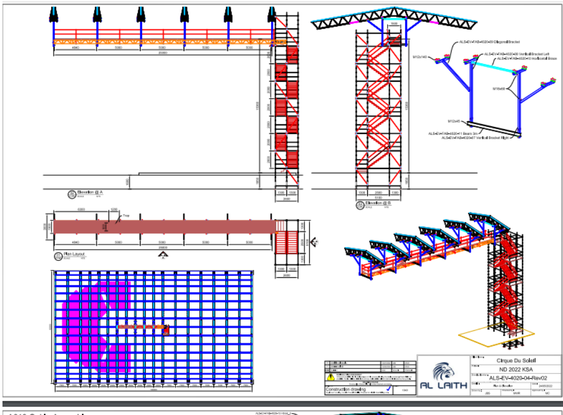
A618 Gable Assembly
